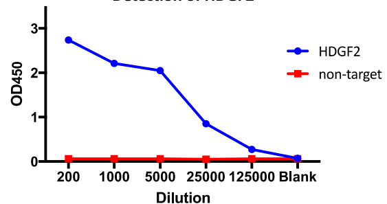
Figure 1: Specificity of anti-HDGF2 (MQR2.1801), determined by ELISA. Antibody diluted in PBS containing 0.05% tween-20 and 1% BSA was tested on human HDGF2 and SA (non-target).
