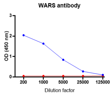
Figure 1: Specificity of anti-WARS (MQR2.3401), determined by ELISA. Antibody stock 0.7 mg/ml diluted in PBS containing 0.05% tween-20 and 1% BSA was tested on human Tryptophanyl-tRNA synthetase (in blue) and non-target protein (in red).
